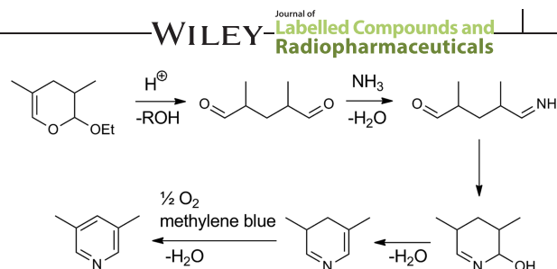
SCHEME 4 Proposed mechanism of the formation of 3,5-dimethylpyridine in analogy to Whaley and Ott 13
